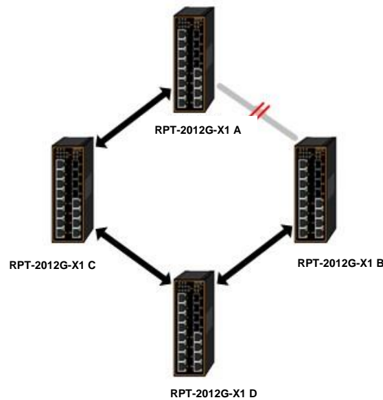
Figure 2.147 Ring Topology for ERPS Setup (Example made on RPT-2012G-X1)
