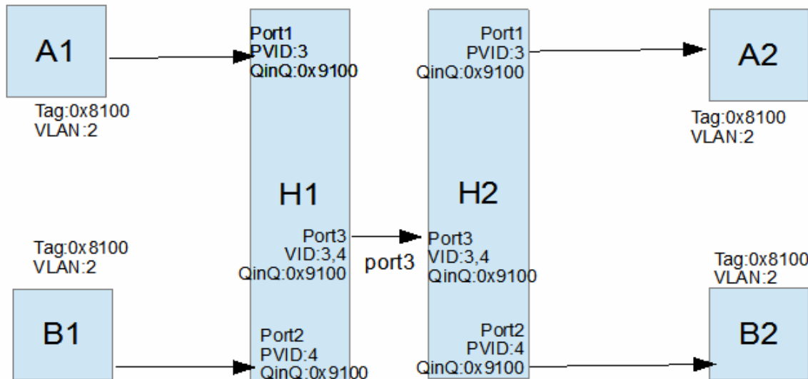
Figure 2.122 Example of Qinq Deployment
