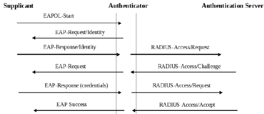
Figure 2.127 RADIUS Authentication Sequence
