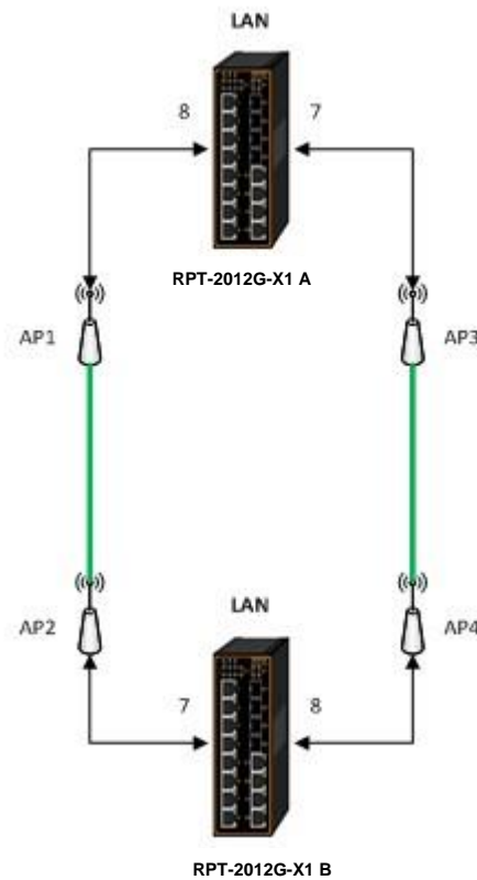
Figure 2.156 Example 2 of Two Wired Bridge U-ring (Example on RPT-2012G-X1)
