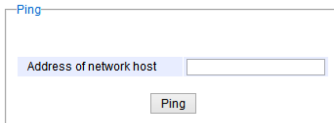
Figure 2.19 Ping Webpage
