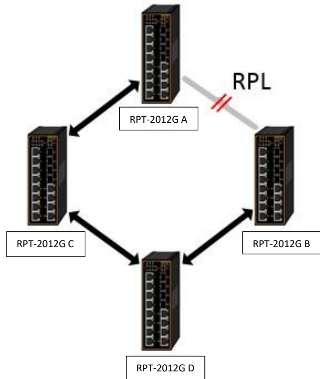
Figure 2.143 An Example of Ring Topology (Example made on RPT-2012G-4F-X1)
