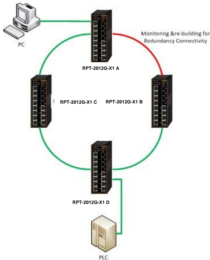
Figure 2.152 iA-Ring Example Topology (Example made on RPT-2012G-X1)
