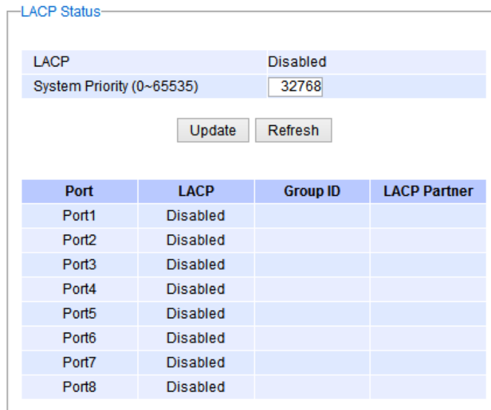
Figure 2.67 LACP Webpage
