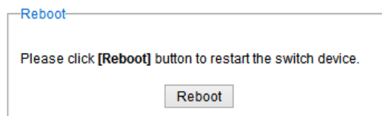
Figure 2.193 Reboot Webpage
