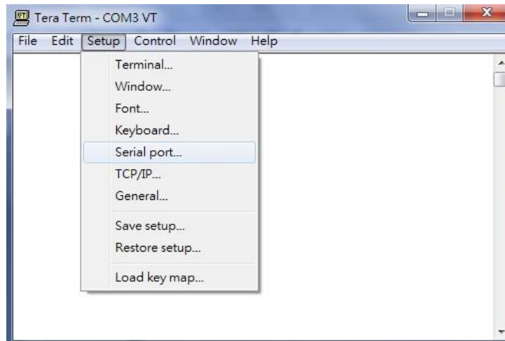
Figure 3.2 Setup Menu
