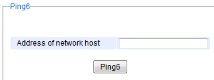
Figure 2.23 Ping6 Webpage
